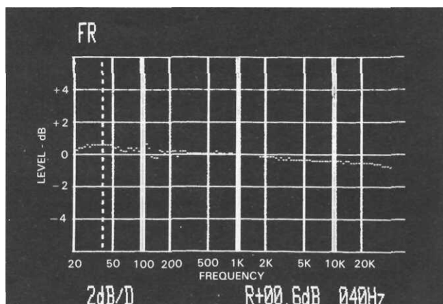
Fig. 12—Expanded-scale phono response, using inverse RIAA input test signal
